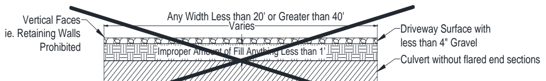
Section A-A (Improperly Installed Driveway) Prohibitive under N.D.C.C. Section 24-05-21
